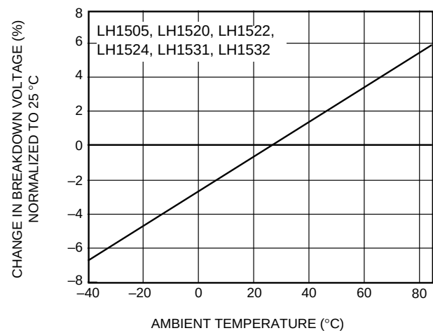
D. Switch Breakdown Voltage vs. Temperature
