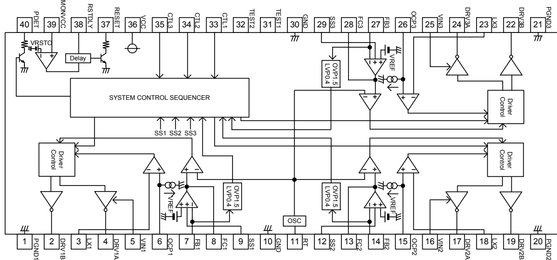
Figure 1 Block char
