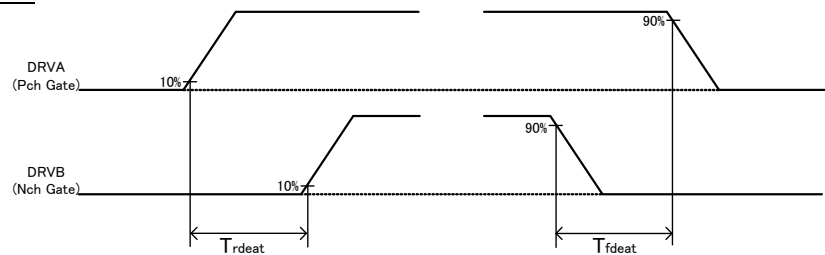
Figure 14 Dead time
