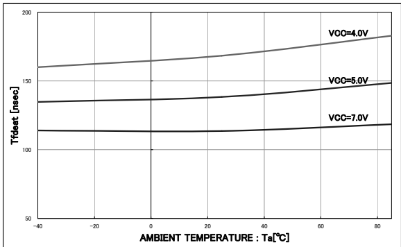
Figure 16 Dead time Tfdead - Temperature characteristic
