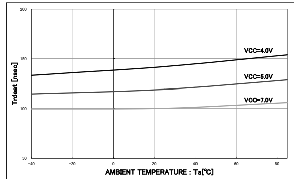
Figure 15 Dead time Trdead - Temperature characteristic
