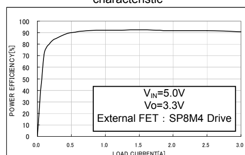
Figure 13 Efficiency
