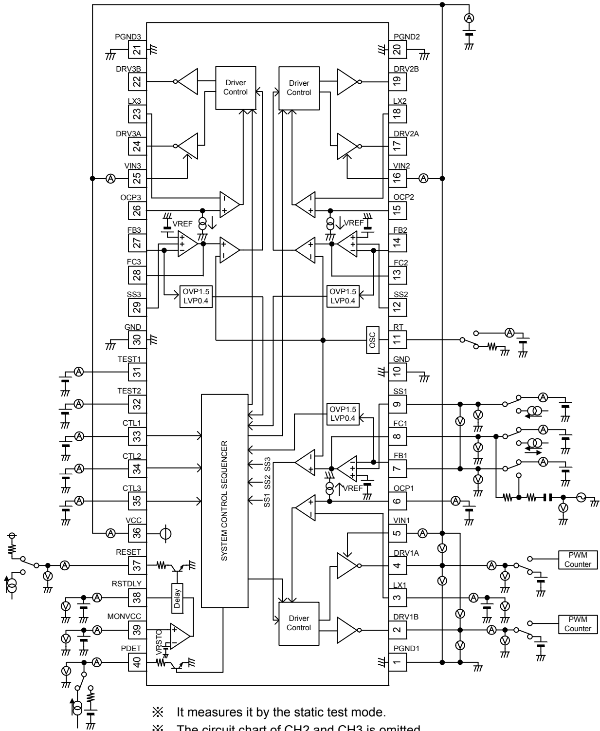
Figure 2 Circuit chart
