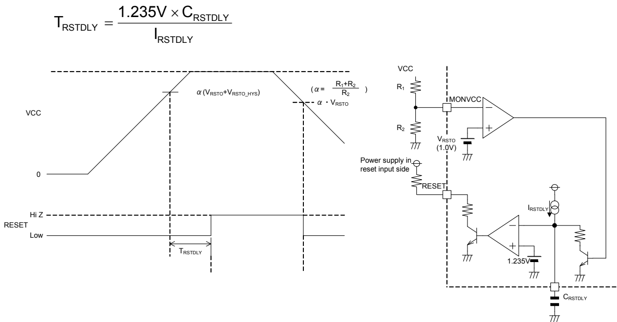
Figure 24 Reset operation
