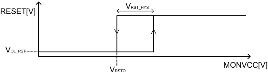
Figure 20 Reset detection
