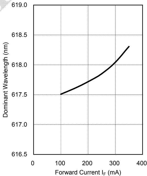
Fig 5. Wavelength Shift
