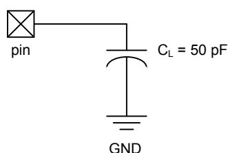
Figure 16-1. Load Conditions
