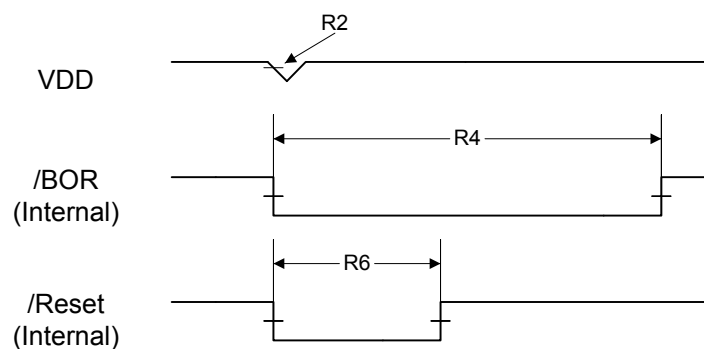
Figure 16-7. Brown-Out Reset Timing
