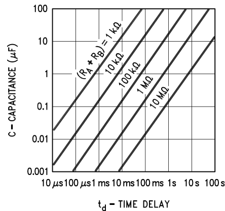
FIGURE 3. Time Delay
