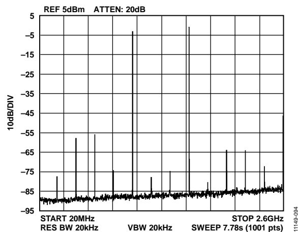
Figure 87. Single-Tone Spectrum at f_{OUT} = 1600 MHz
