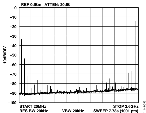
Figure 84. Single-Tone Spectrum at f_{OUT} = 2350 MHz
