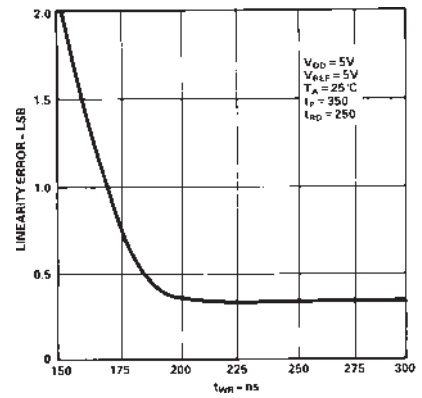
TPC 3. Accuracy vs. t_{WR}
