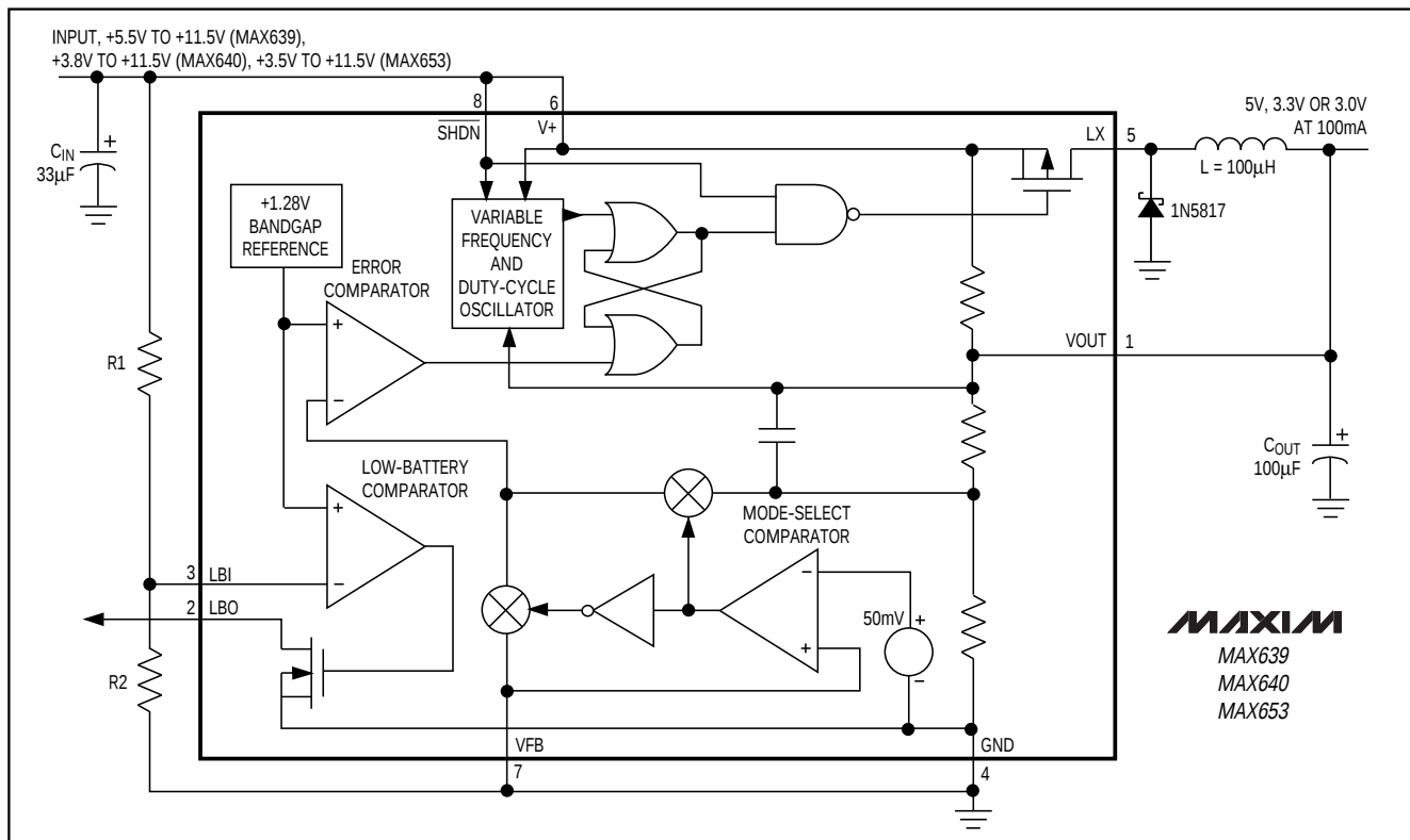
Figure 3. Block Diagram
