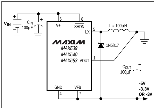
Figure 6. Inverting Configuration
