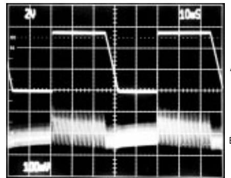
MAX639 LINE-TRANSIENT RESPONSE
