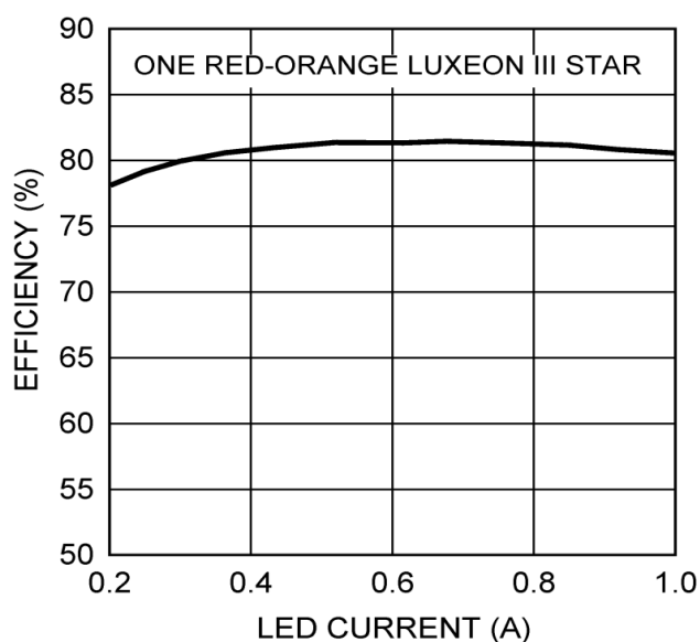
Efficiency vs LED Current ( V_{IN} = 5 V)
