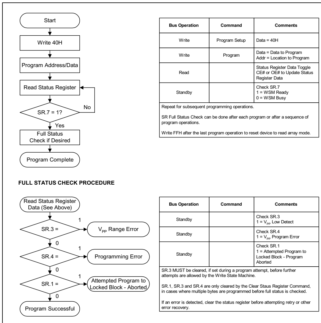
Figure 12. Program Flowchart
