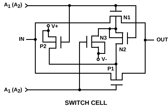
SWITCH CELL
