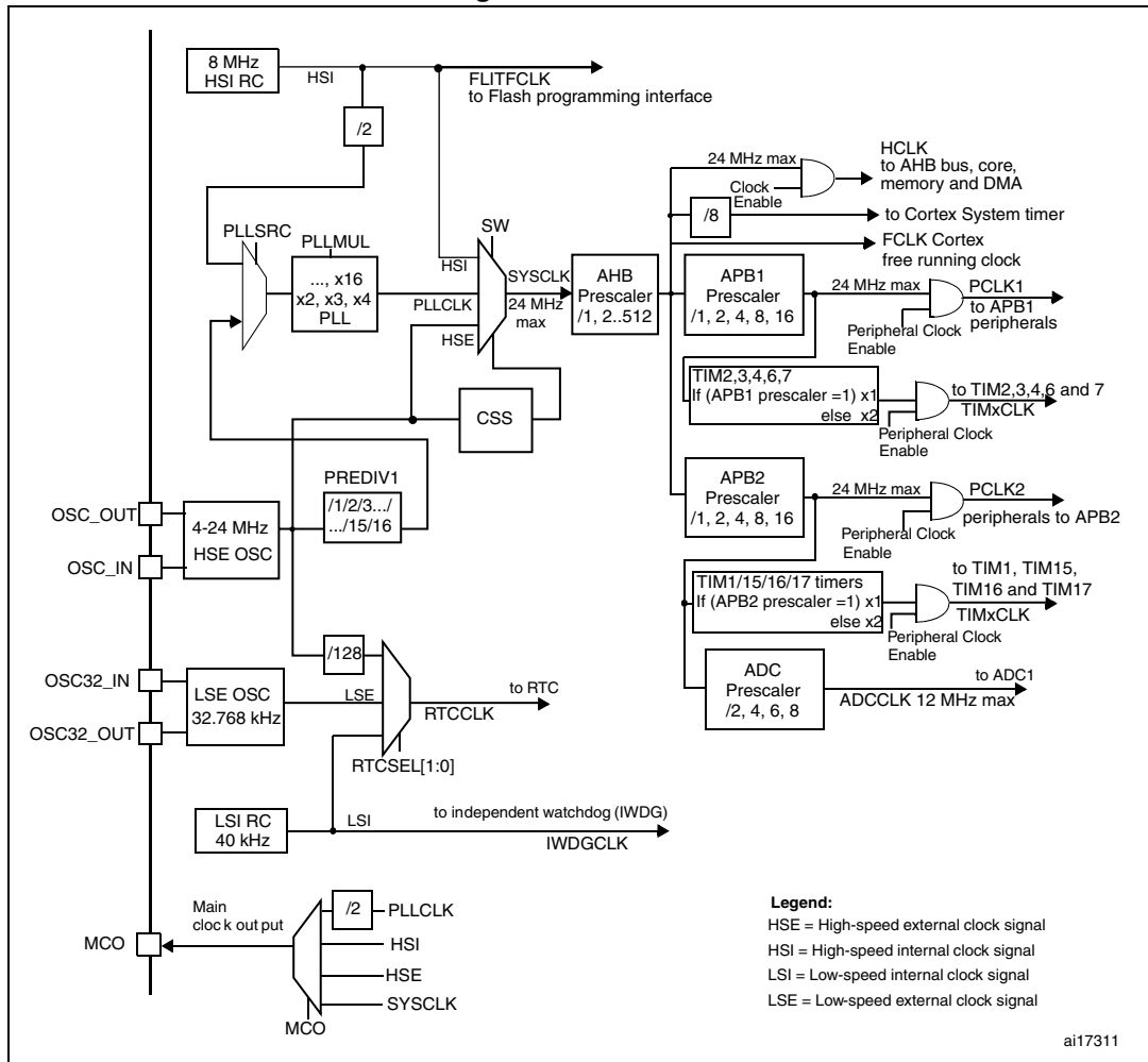
Figure 2. Clock tree
