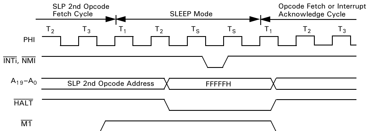
Figure 14. SLEEP Timing
