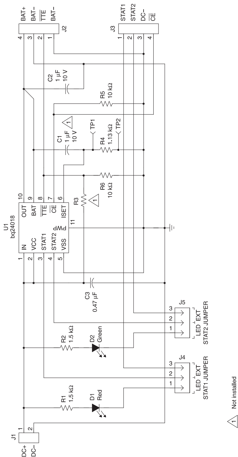
Figure 1. EVM Schematic Diagram
