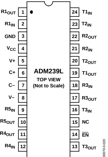
Figure 10. ADM239L PDIP/CERDIP/SOIC Pin Configuration
