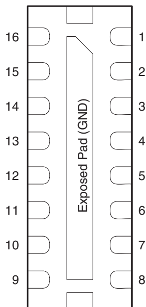
DFN-16 (Bottom View)
