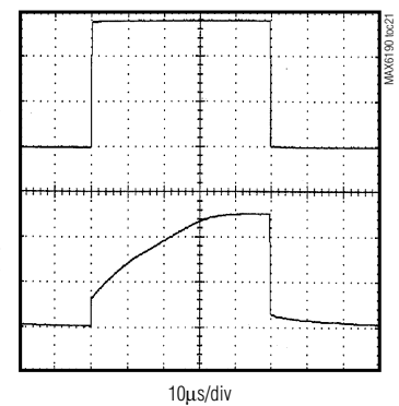
MAX6195 TURN-ON TRANSIENT
