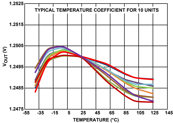
FIGURE 33. V_{OUT} vs TEMPERATURE
