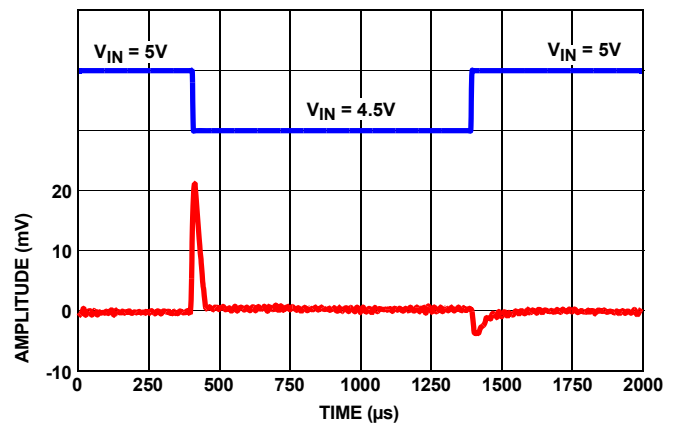
FIGURE 24. LINE TRANSIENT RESPONSE WITH 10µF LOAD
