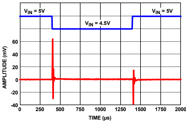
FIGURE 23. LINE TRANSIENT RESPONSE WITH 0.1µF LOAD
