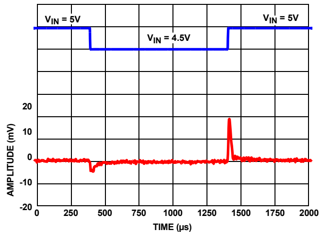
FIGURE 7. LINE TRANSIENT RESPONSE WITH 10µF LOAD
