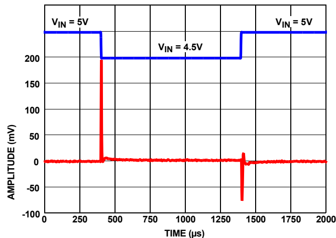
FIGURE 125. LINE TRANSIENT RESPONSE WITH 0.1\mu F LOAD
