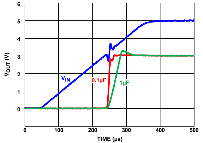
FIGURE 96. TURN-ON TIME
