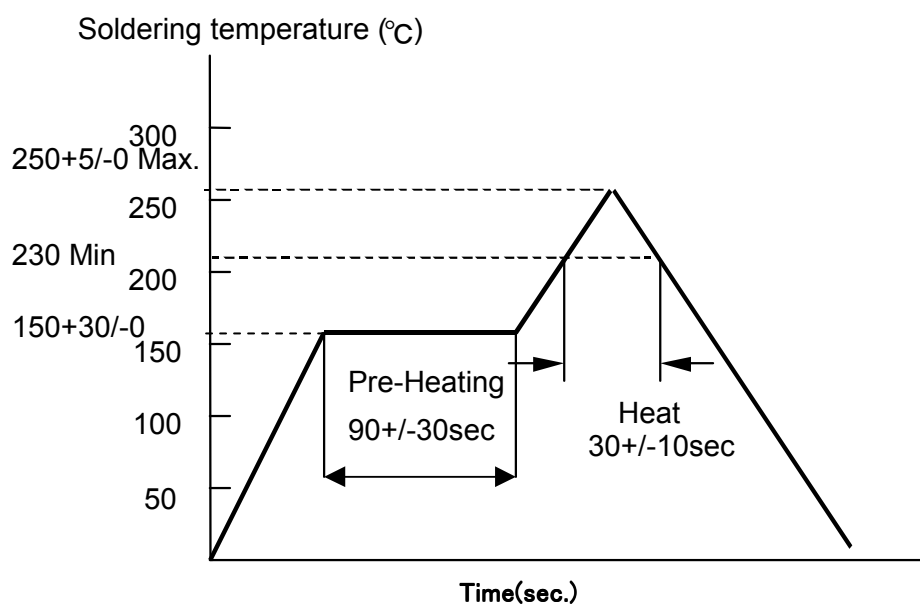
Figure 3 Temperature profile of reflow soldering
