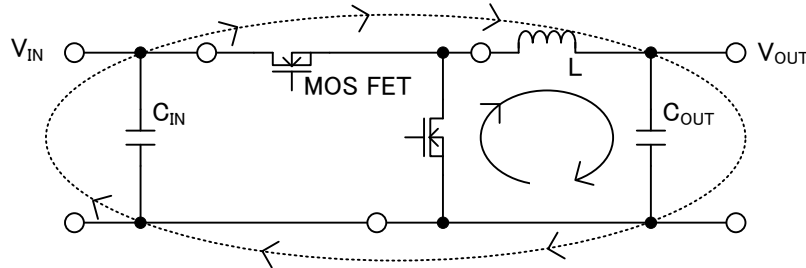
Figure 27. Current Loop of Buck Converter
