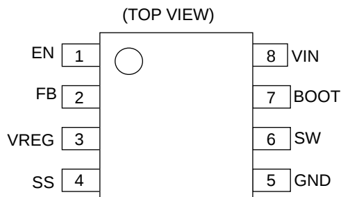
Figure 2. Pin Assignment
