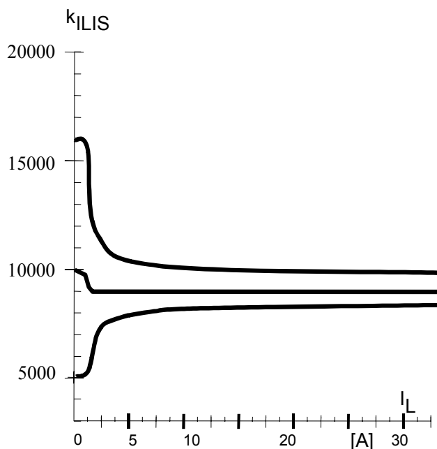
Figure 6b: Current sense ratio 22 :
