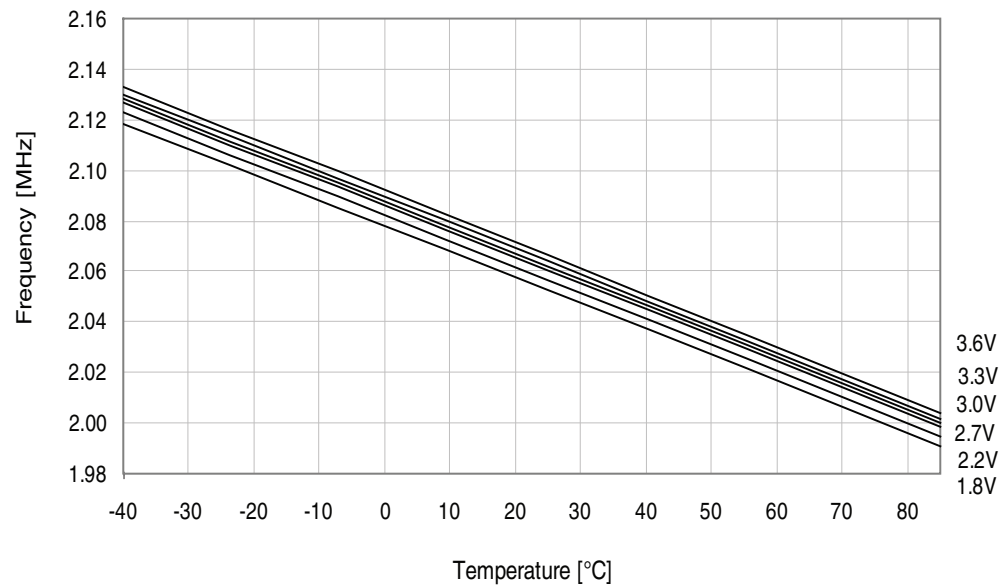
Figure 37-329. 2MHz internal oscillator frequency vs. temperature. DFLL enabled, from the 32.768kHz internal oscillator.
