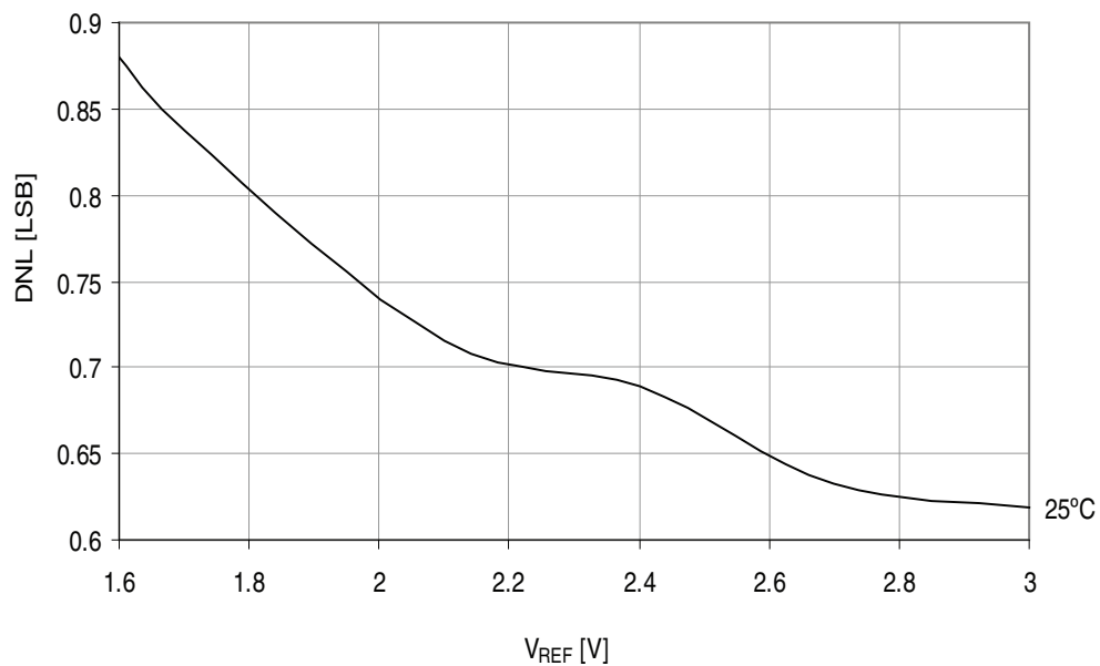
Figure 37-50. DNL error vs. V_{REF} .
