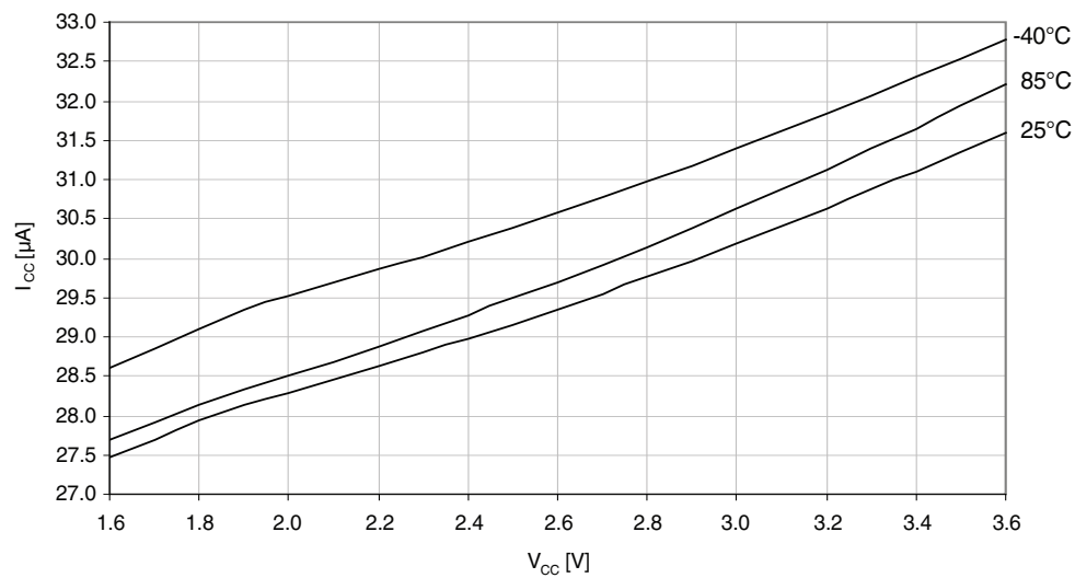
Figure 37-95. Idle mode supply current vs. V_{\text{CC}} .
