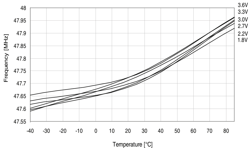
Figure 37-335. 48MHz internal oscillator frequency vs. temperature. DFLL enabled, from the 32.768kHz internal oscillator.
