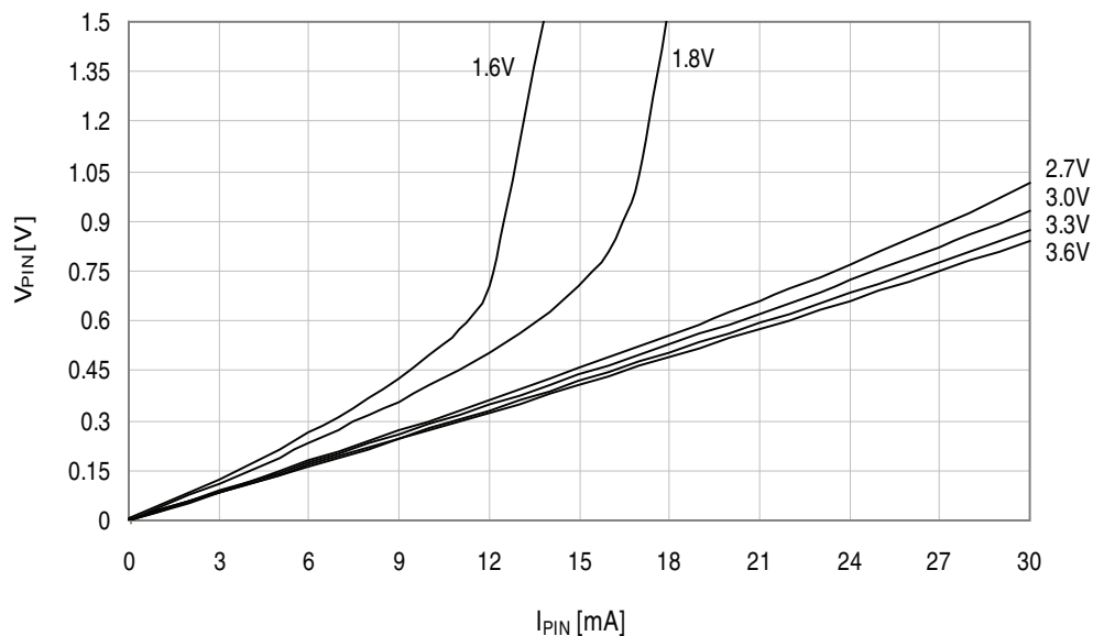
Figure 37-286. I/O pin output voltage vs. sink current.
