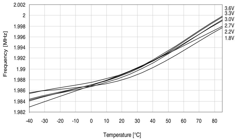
Figure 37-329. 2MHz internal oscillator frequency vs. temperature. DFLL enabled, from the 32.768kHz internal oscillator.
