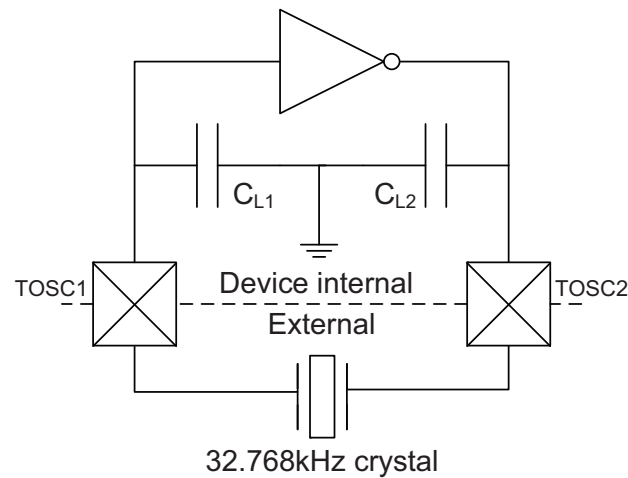
Figure 36-11.TOSC input capacitance.
