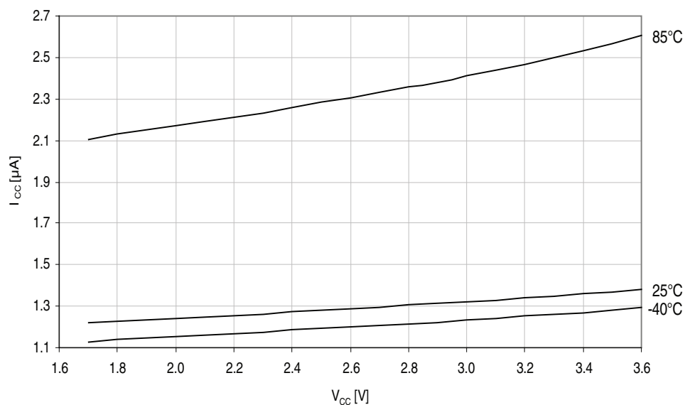
Figure 37-102. Power-down mode supply current vs. V_{CC} . Watchdog and sampled BOD enabled.
