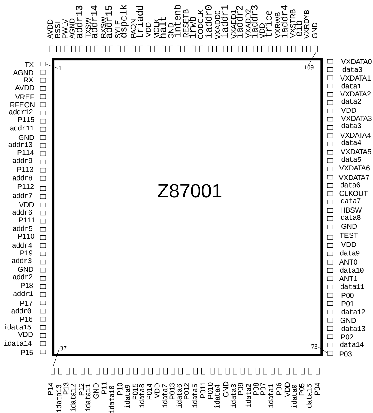
Figure 3. 144 Pin QFP Pin Configuration
