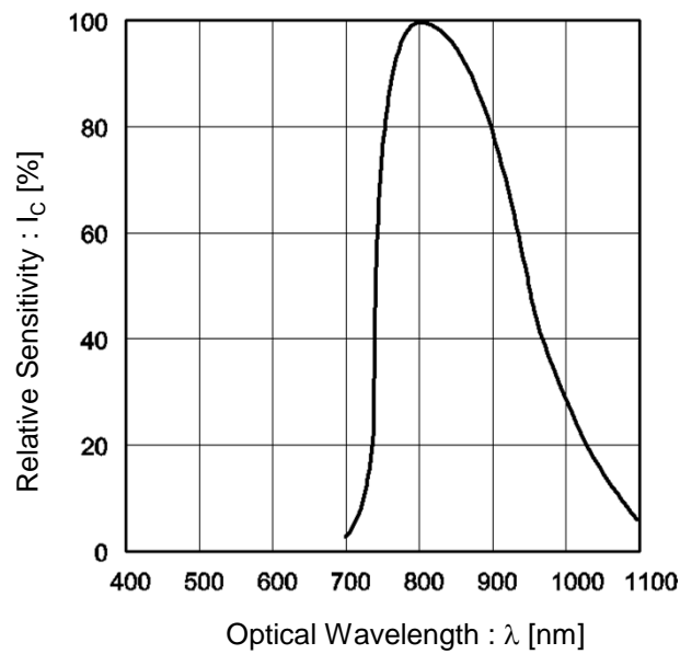
Fig.5 Spectral Sensitivity
