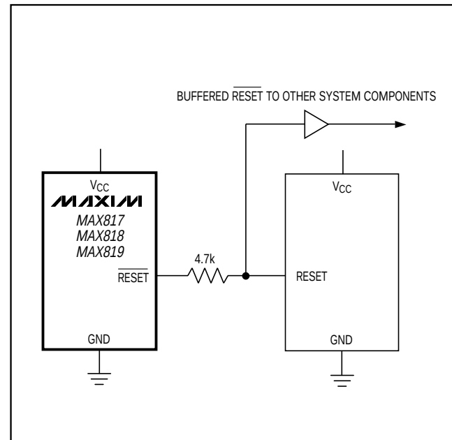
Figure 14. Interfacing to \mu Ps with Bidirectional Reset I/O
