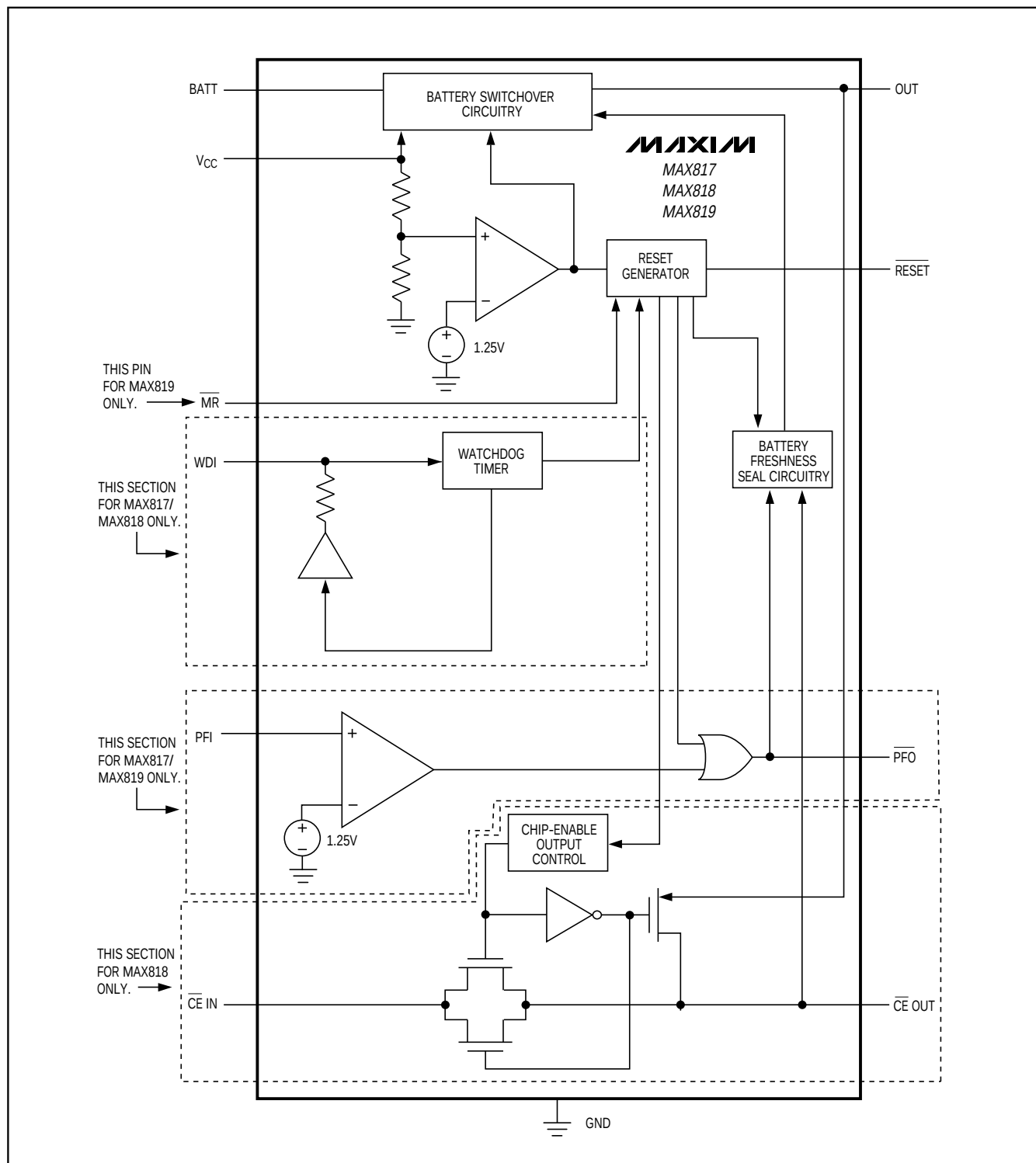
Figure 1. Functional Diagram
