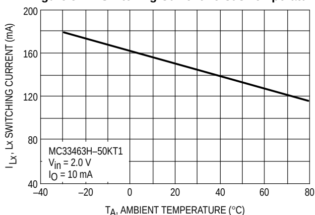
Figure 5. Lx Switching Current versus Temperature
