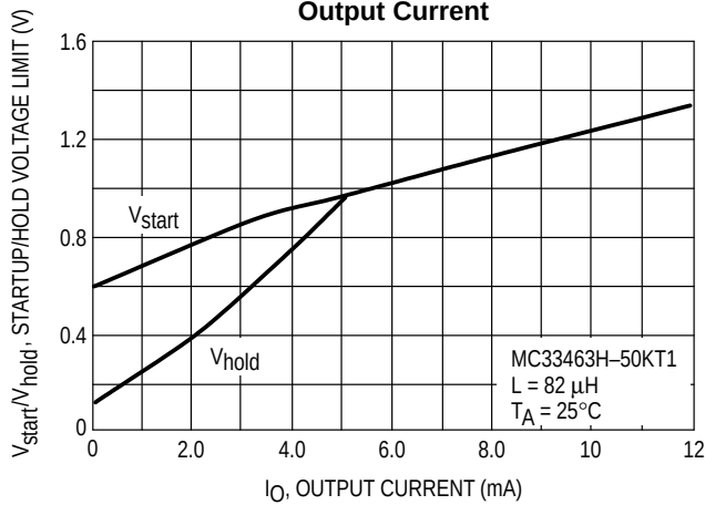
Figure 11. Startup/Hold Voltage versus Output Current
