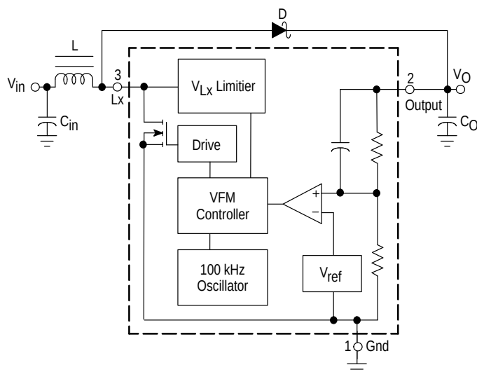
MC33463H-XXLT1
