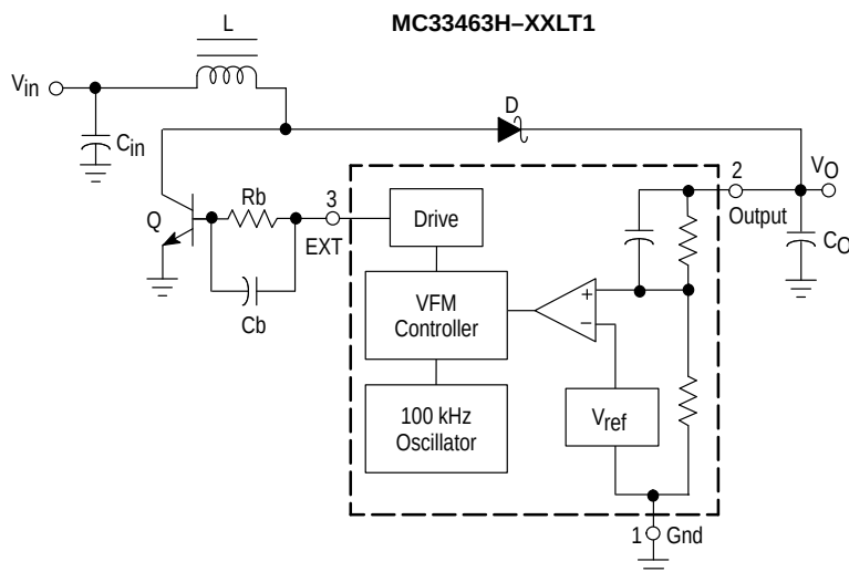
MC33463H-XXLT1
