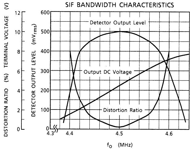
SIF BANDWIDTH CHARACTERISTICS
