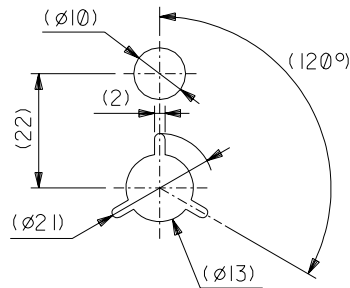
DETAIL "G"
