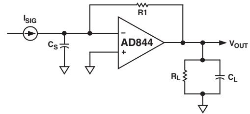
Figure 3. Current-to-Voltage Converter
