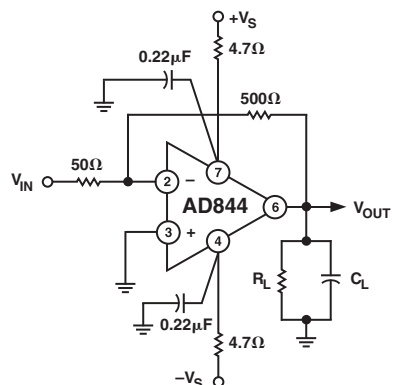
TPC 15. Gain of -10 Amplifier
