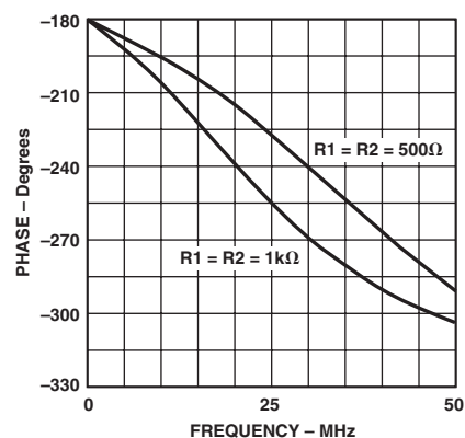
TPC 12. Phase vs. Frequency for Gain = -1 , R_L = 500\Omega , C_L = 0\text{ pF}
