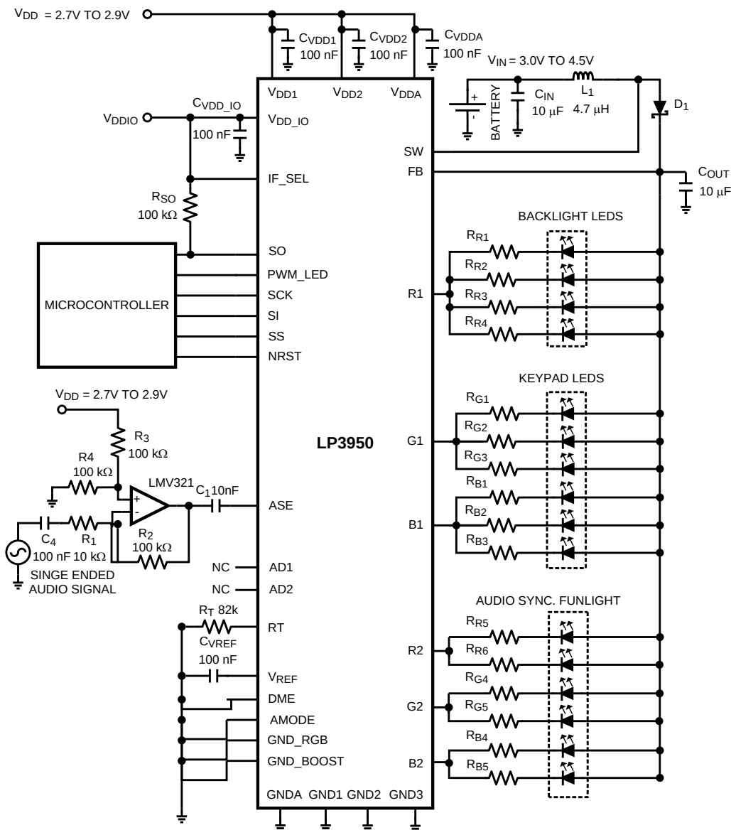
Figure 34. Backlight and Keypad LEDs Controlled by the Pattern Generator Funlight LEDs Controlled by Audio Synchronization
