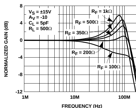
FIGURE 4. INVERTING FREQUENCY RESPONSE FOR VARIOUS R_F
