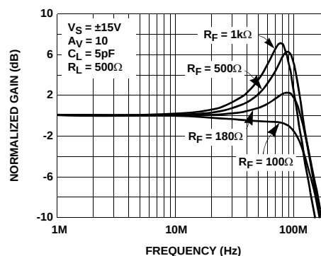
FIGURE 2. NON-INVERTING FREQUENCY RESPONSE FOR VARIOUS R_F
