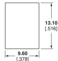
Recommended Panel Cutout Max. Panel Thk. 1.7 [0.067]
