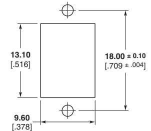
Recommended Panel Cutout Max. Panel Thk. 1.7 [0.067]
