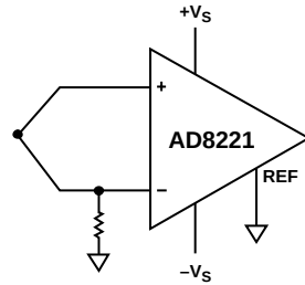
THERMOCOUPLE
