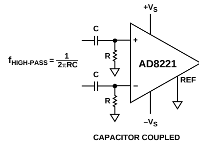
CAPACITOR COUPLED
