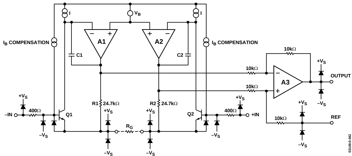
Figure 42. Simplified Schematic
