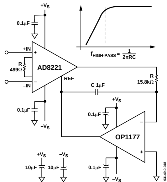
Figure 52. AC-Coupled Circuit
