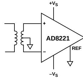
TRANSFORMER
