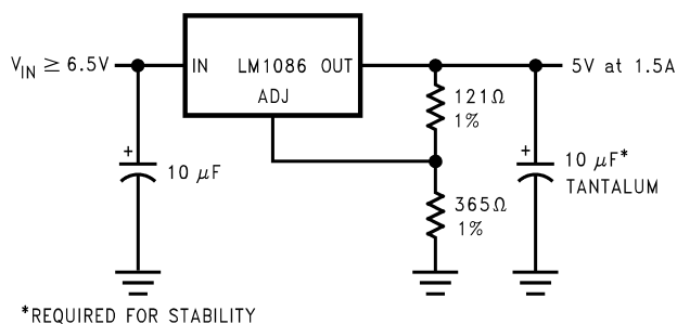
Figure 26. Adjustable @ 5V
