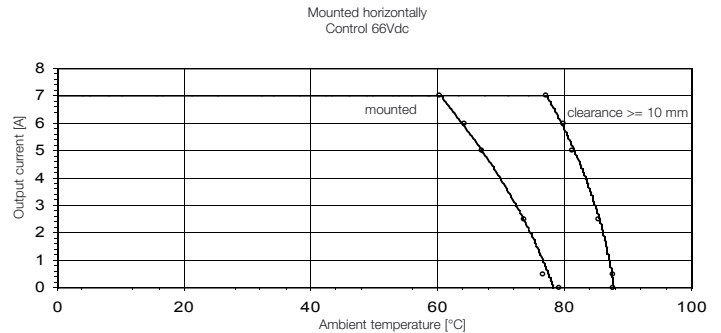
WRS 1 24/60 VUC • 8418210000
