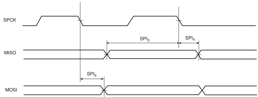
Figure 11-5. SPI Master mode with (CPOL=0 and NCPHA=1) or (CPOL=1 and NCPHA=0)
