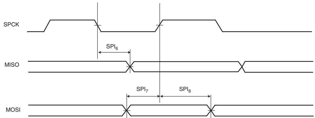
Figure 11-6. SPI Slave mode with (CPOL=0 and NCPHA=1) or (CPOL=1 and NCPHA=0)
