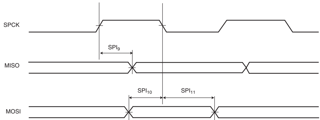
Figure 11-7. SPI Slave mode with (CPOL = NCPHA = 0) or (CPOL= NCPHA= 1)
