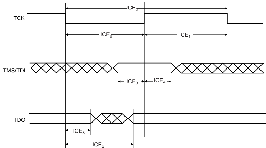
Figure 11-2. ICE Interface Signals
