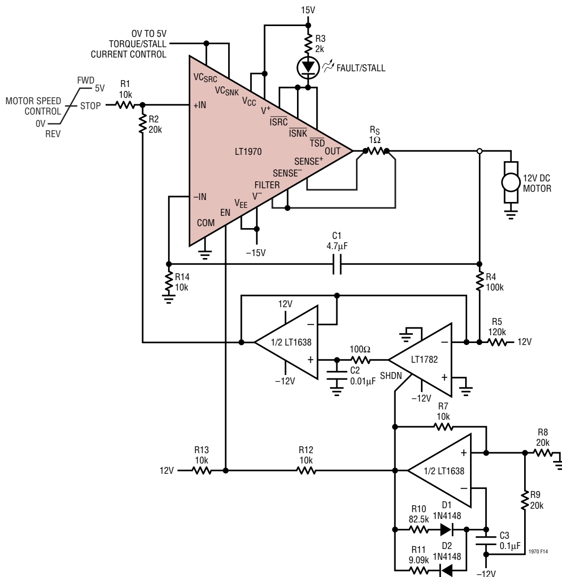
Figure 14. Simple Bidirectional DC Motor Speed Controller Without a Tachometer
