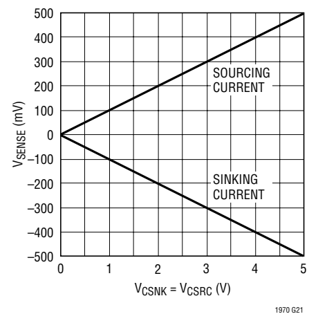
Full Range Current Sense Transfer Curve
