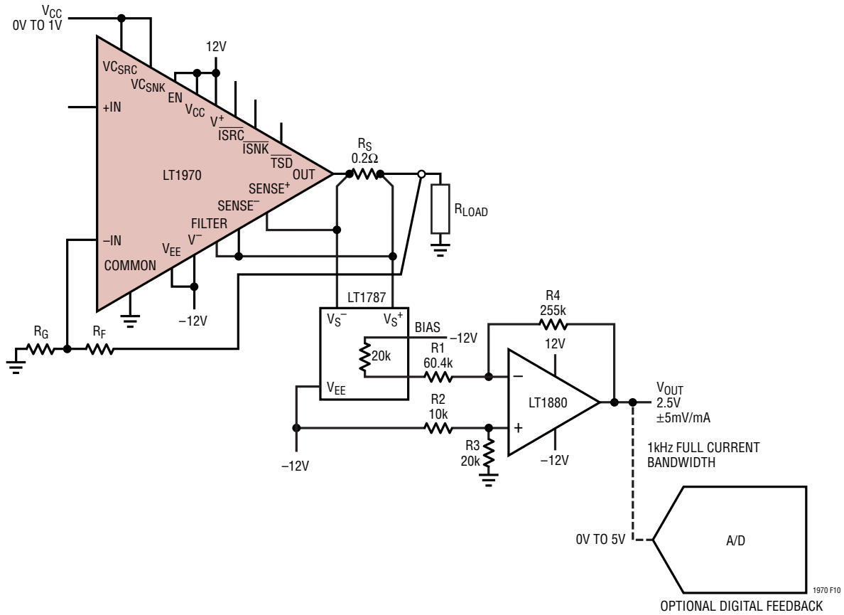
Figure 10. Sensing Output Current
