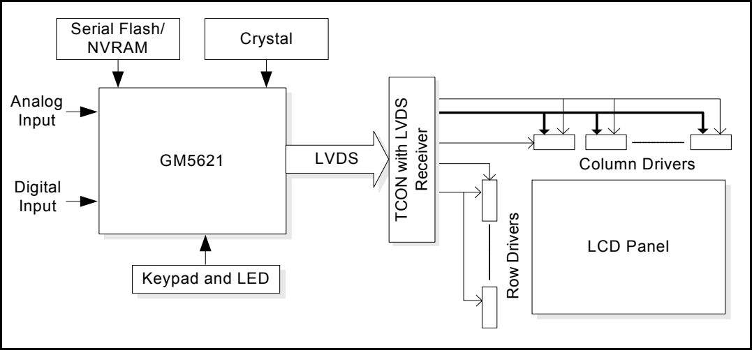
Figure 1. GM5621 system design: conventional interface
