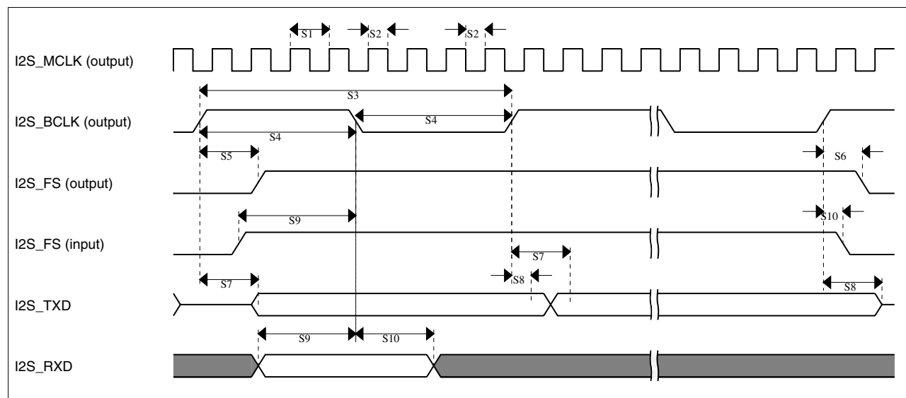
Figure 31. I 2 S timing — master mode
