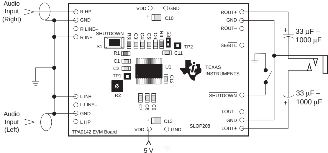
Figure 3–10. TPA0142 EVM Connected for Stereo Single-Ended Output
