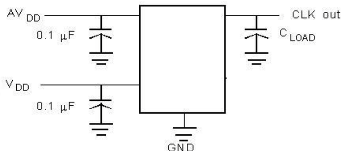
Figure 7. Test Circuit
