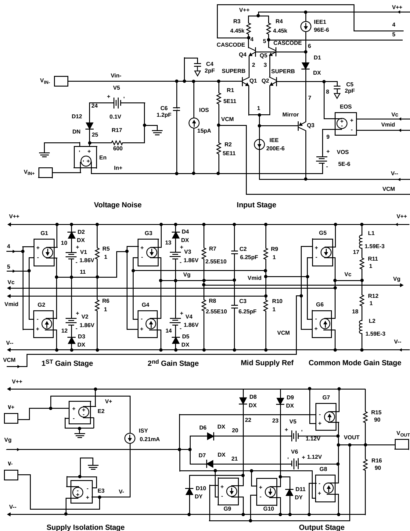
FIGURE 56. SPICE SCHEMATIC
