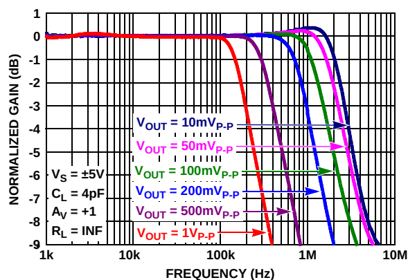
FIGURE 46. GAIN vs FREQUENCY vs OUTPUT VOLTAGE
