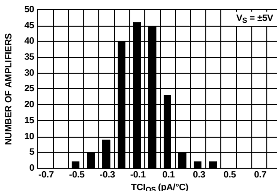
FIGURE 20. TC_{1OS-} vs NUMBER OF AMPLIFIERS, V_S = \pm 5V
