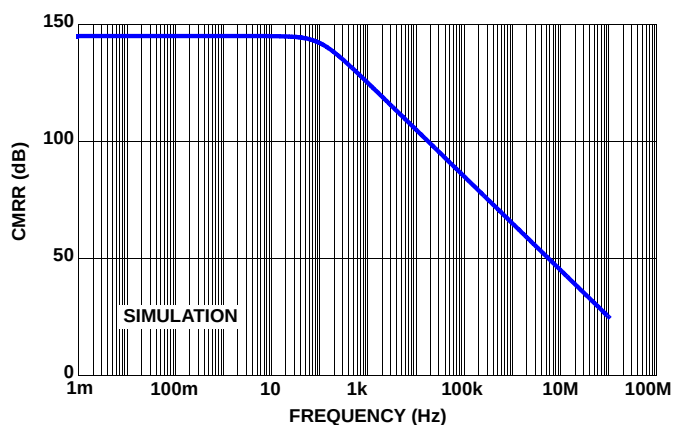
FIGURE 68. SIMULATED CMRR vs FREQUENCY
