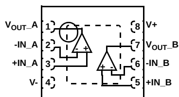
ISL28207 (8 LD TDFN) TOP VIEW
