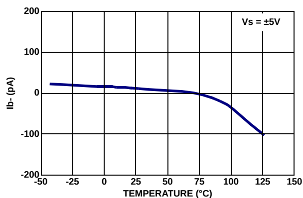
FIGURE 14. NEGATIVE BIAS CURRENT vs TEMPERATURE, V_S = \pm 5V
