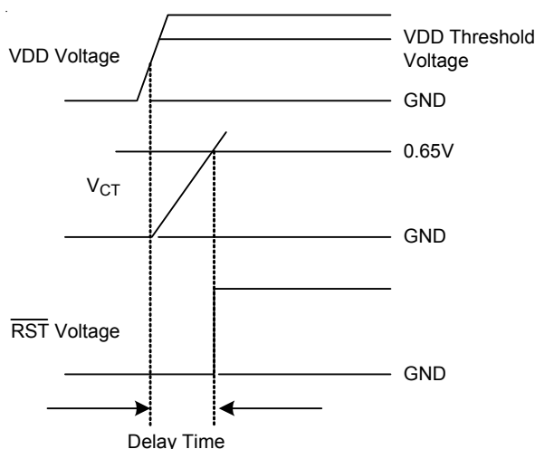
Figure 1. Delay Time
