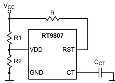
Figure 2. Voltage Divider
