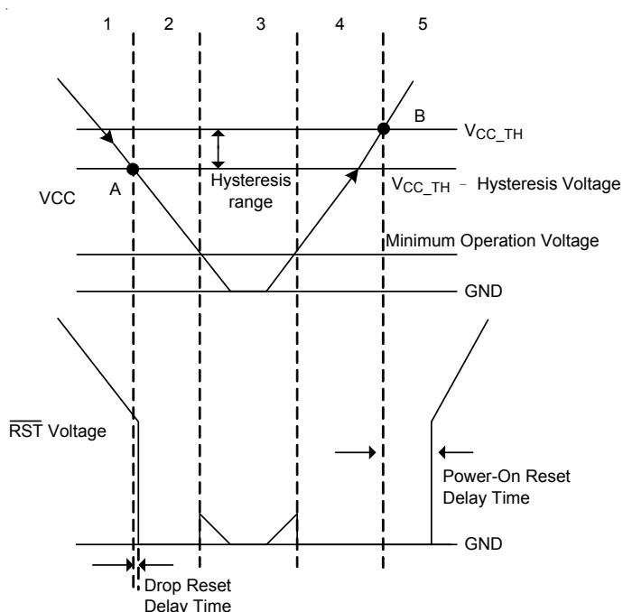
Figure 3. Operation Diagram
