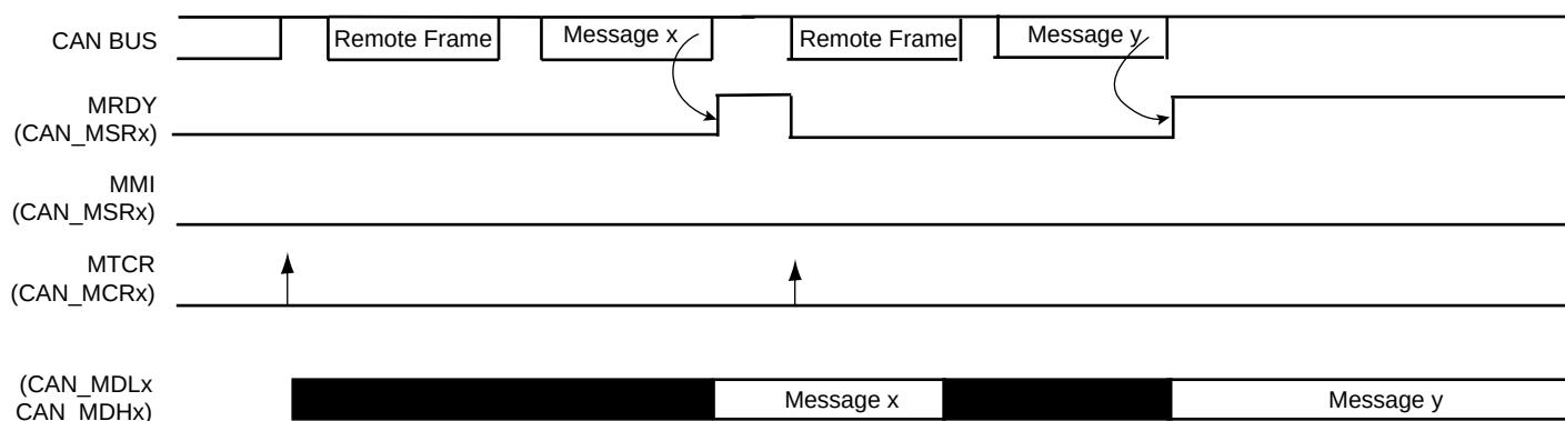
Figure 38-18. Consumer Handling
