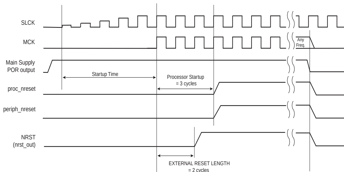
Figure 13-4. Power-up Reset
