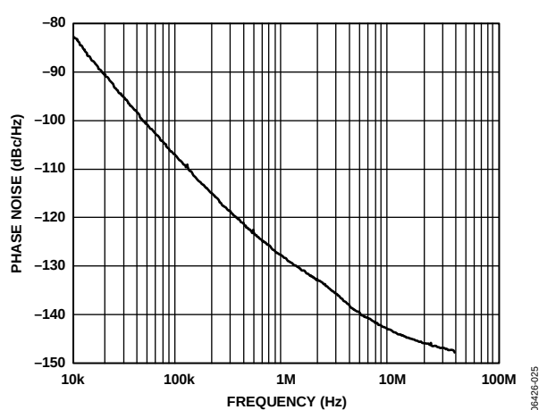
Figure 30. Internal VCO Phase Noise (Absolute) Direct to LVPECL at 2050 MHz
