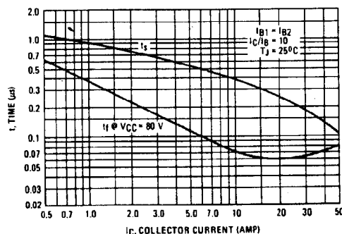
FIGURE 4 - TURN OFF TIME
