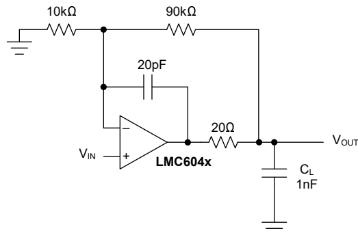
Figure 6-2. LMC604x Noninverting Gain-of-10 Amplifier, Compensated to Handle Capacitive Loads
