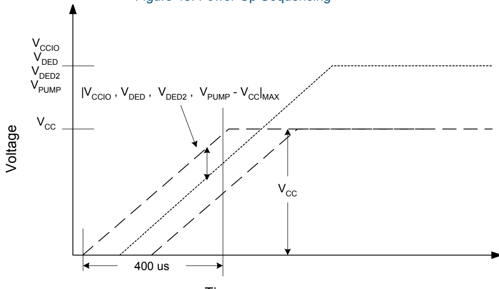
Figure 45: Power-Up Sequencing
