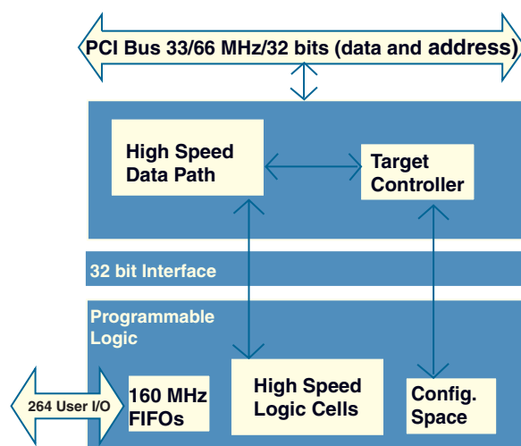
Figure 1: QL58x0 Block Diagram
