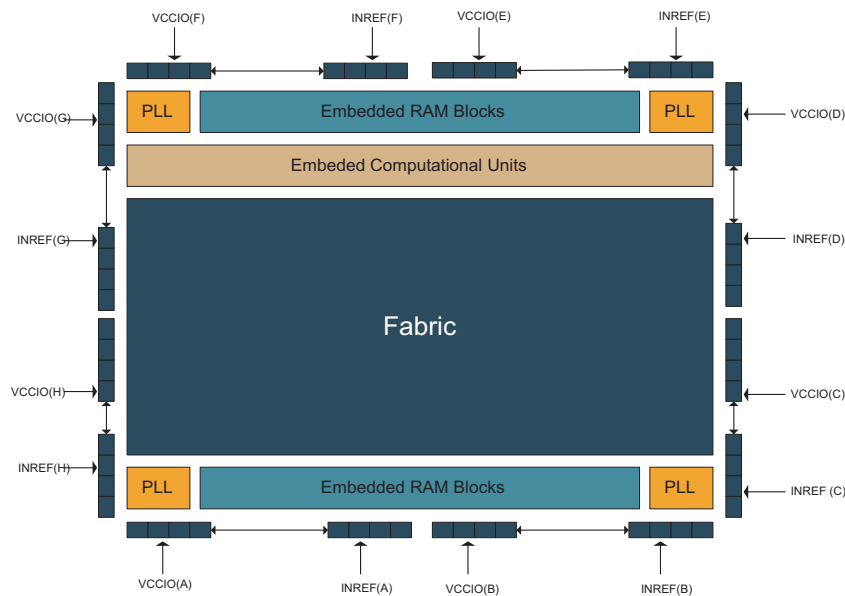
Figure 9: Multiple I/O Banks on QL5842 and QL5832
