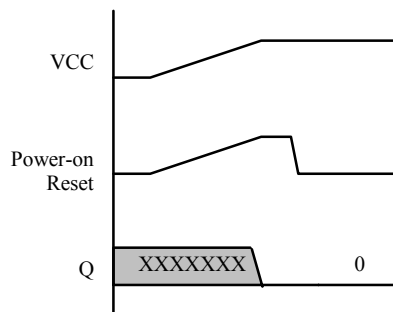
Figure 15: Power-On Reset
