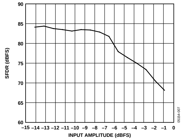
Figure 6. Single-Tone SFDR vs. AIN with f_{IN} = 70\text{ MHz}
