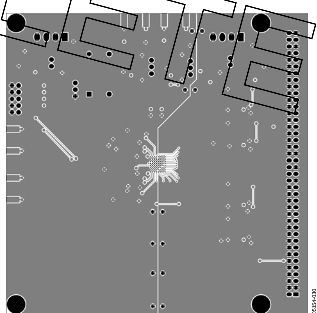
Figure 24. AD15252 Evaluation Board Top Signal
