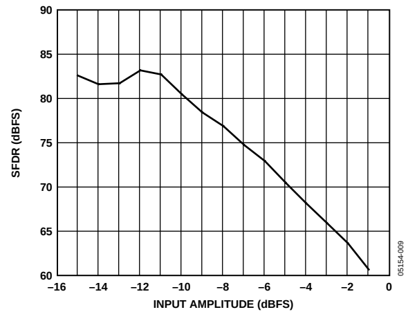
Figure 8. Single-Tone SFDR vs. AIN with f_{IN} = 140\text{ MHz}
