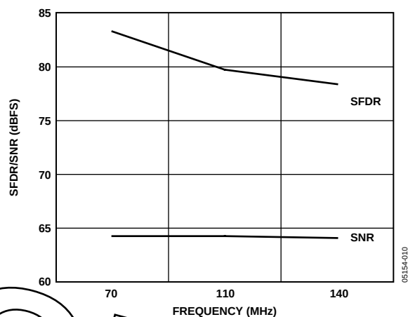
Figure 9. Single-Tone SNR/SEDR vs. f_{IN}
