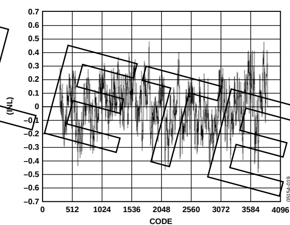
Figure 13. Typical INL
