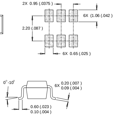
RECOMMENDED FOOTPRINT
